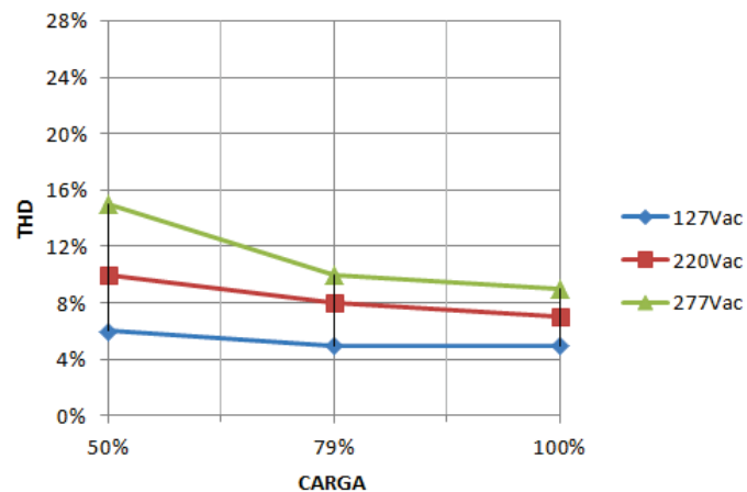
L4014-CIP4U1050/150P ( I_o=0,7A )
