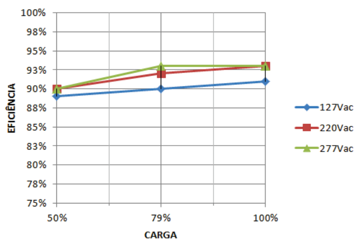
L4014-CIP4U1050/150P ( I_o=0,7A )
