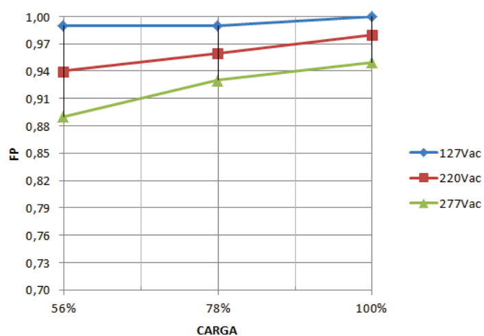
L4015-CIP4U1500/150P ( I_o=1,05A )
