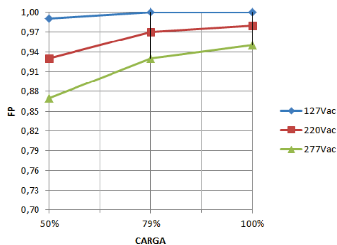
L4014-CIP4U1050/150P ( I_o=0,7A )
