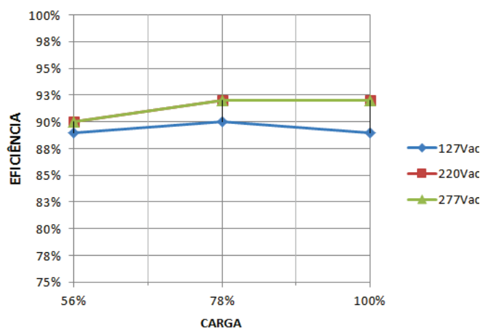
L4015-CIP4U1500/150P ( I_o=1,05A )
